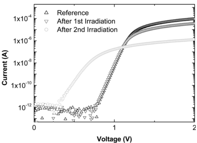
Fig. 2. Current-voltage characteristic at room temperature after irradiated with neutrons.
